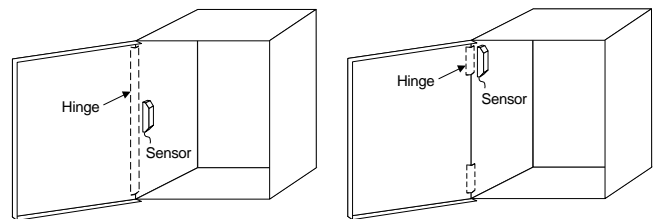
Figure 1. Solid Hinge
