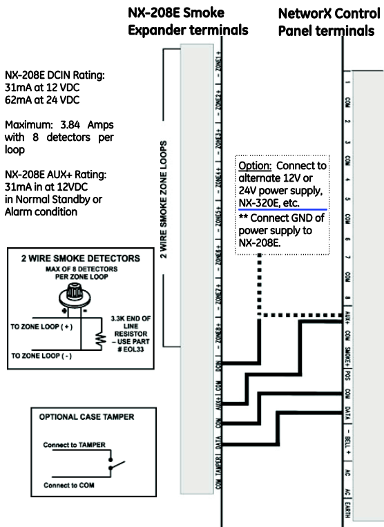
Figure 2: Wiring connections
