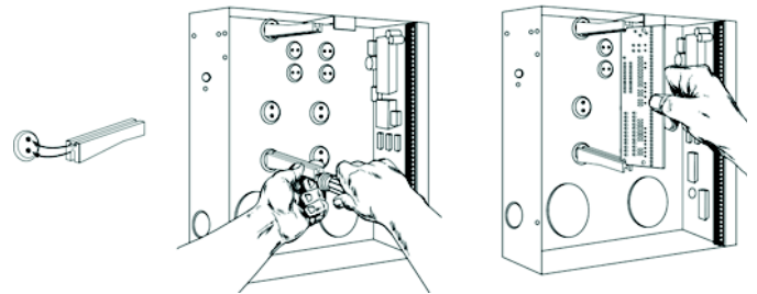
Figure 1: Board installation
