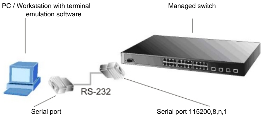
Figure 1: Terminal setup diagram
