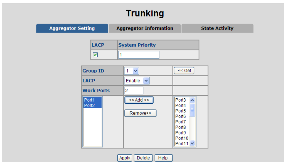
Figure 4-43: Aggregation Information of Switch 1
