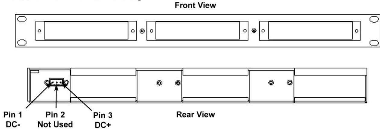
Figure 1: Model 503H Horizontal Card Cage
