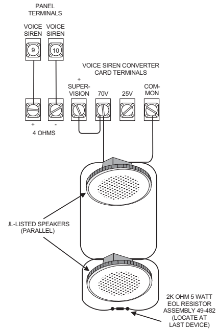
Figure 3: Typical Advent panel card wiring
