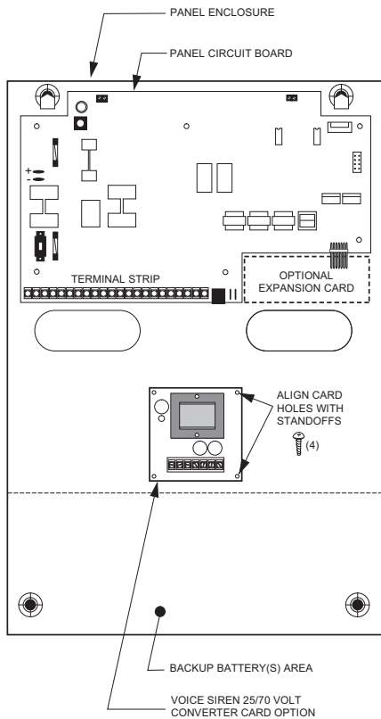
Figure 2: Mounting the card in the Advent panel
