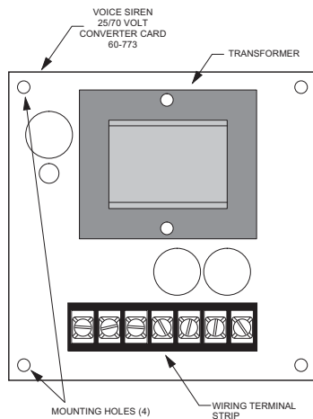
Figure 1: Card components
