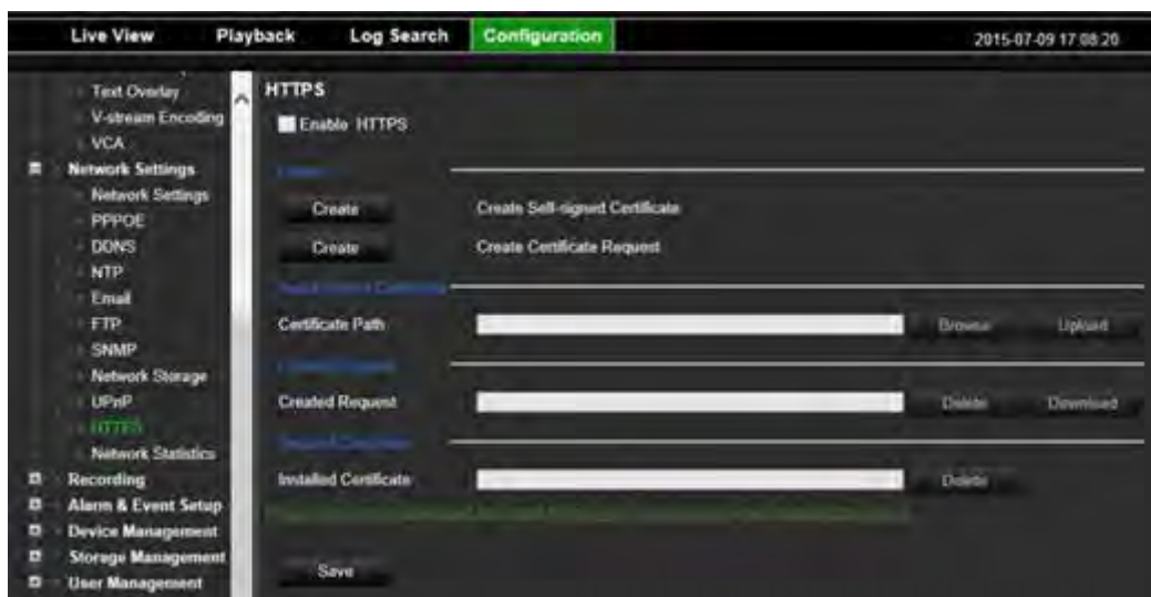
Figure 34: HTTPS configuration screen
