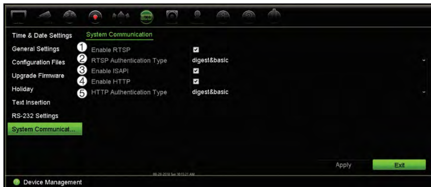
Figure 31: System communication settings window
