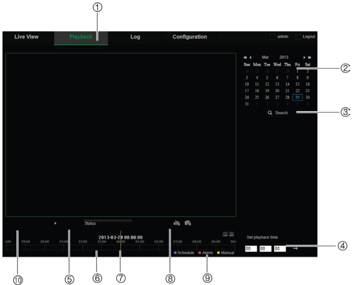
Figure 18: Playback window
