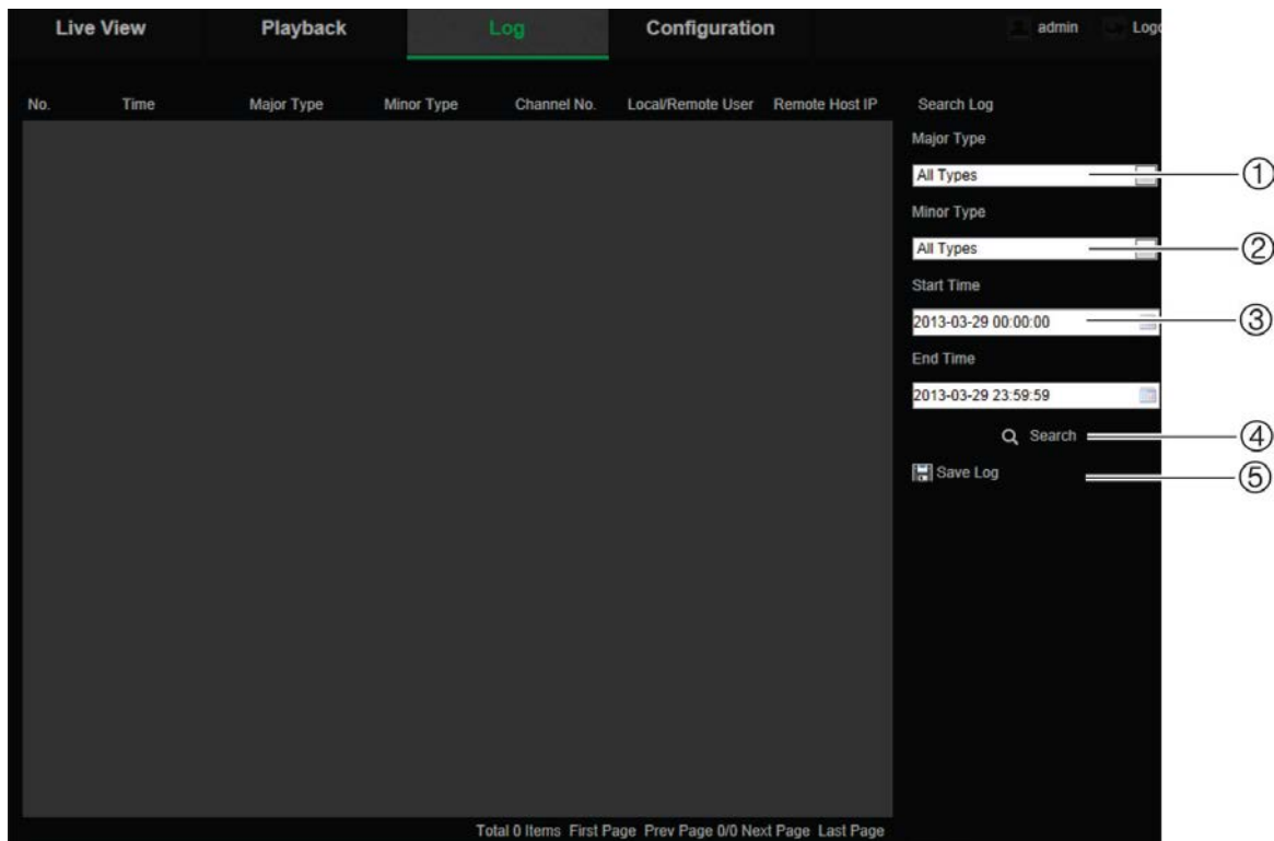
Figure 19: Log window
