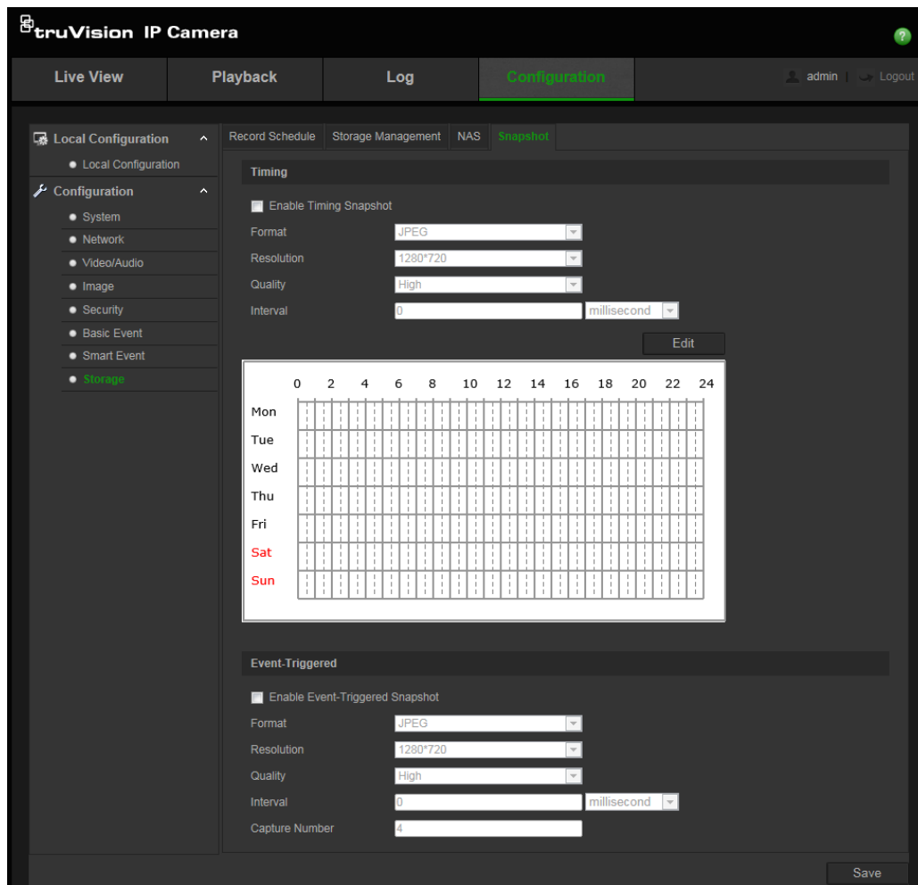
Figure 13: Snapshot menu
