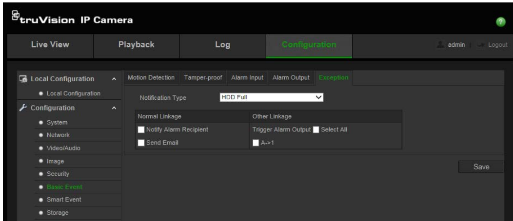
Figure 10: Exception menu
