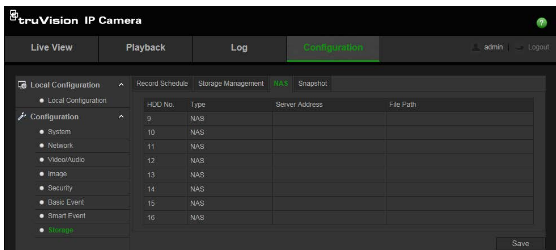
Figure 14: NAS menu
