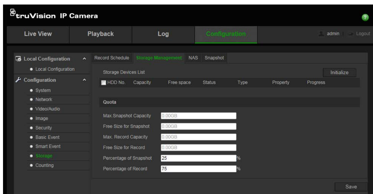
Figure 18: Storage window
