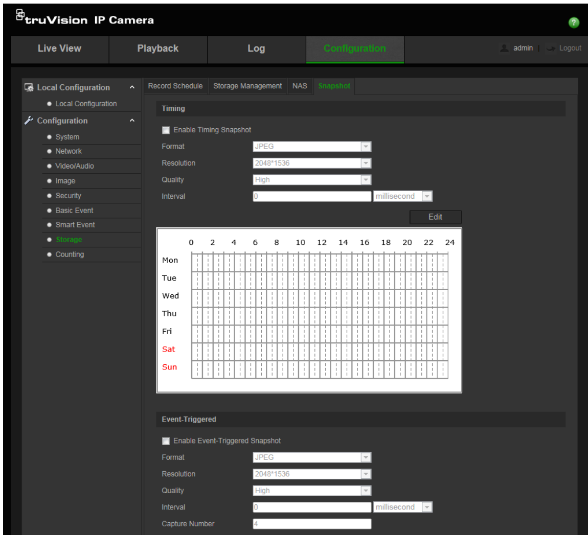
Figure 21: Snapshot menu
