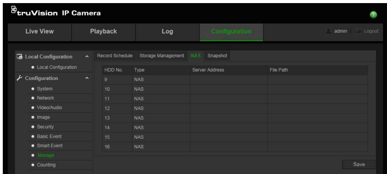
Figure 22: NAS menu
