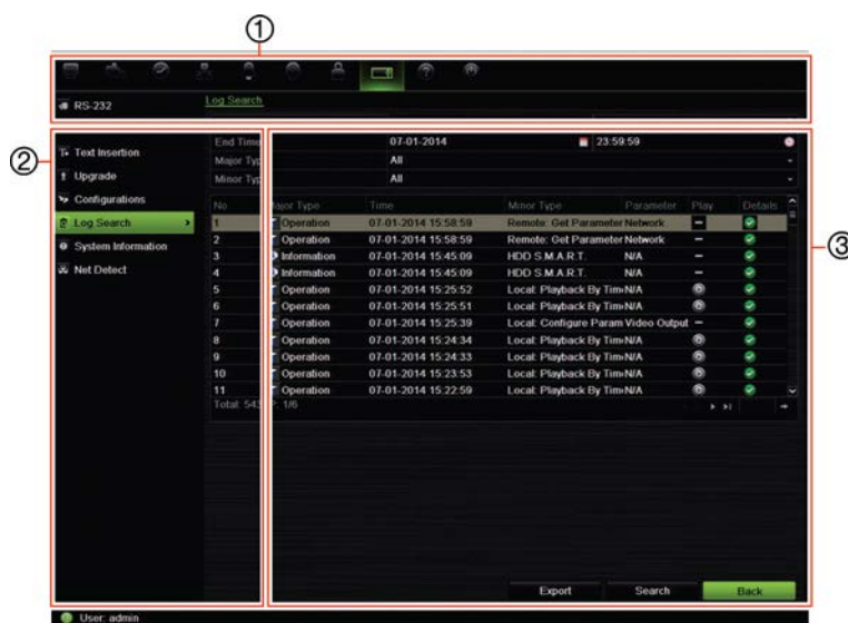
Figure 10: Menu structure
