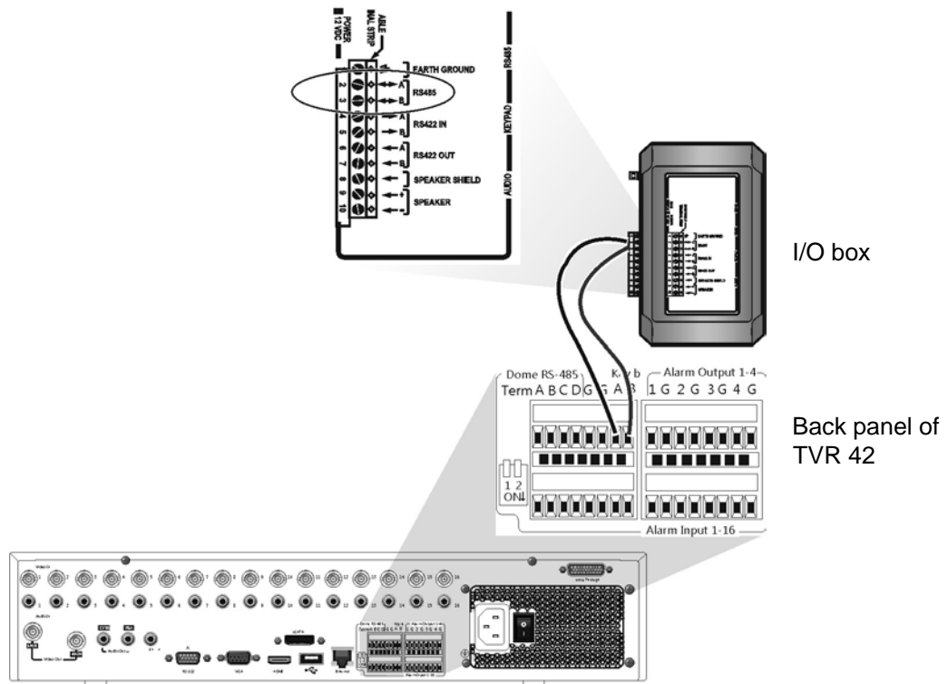
Figure 41: Keypad and DVR connections
