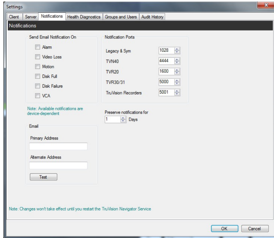
Figure 57: Notification tab
