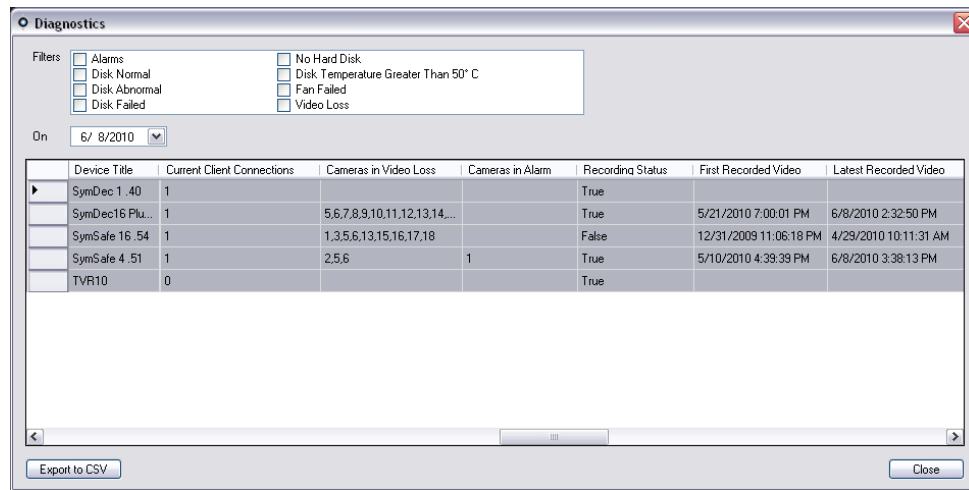
Figure 60: Diagnostics Window
