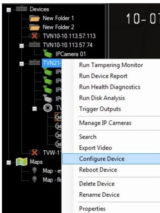
Figure 40: Configure Device
