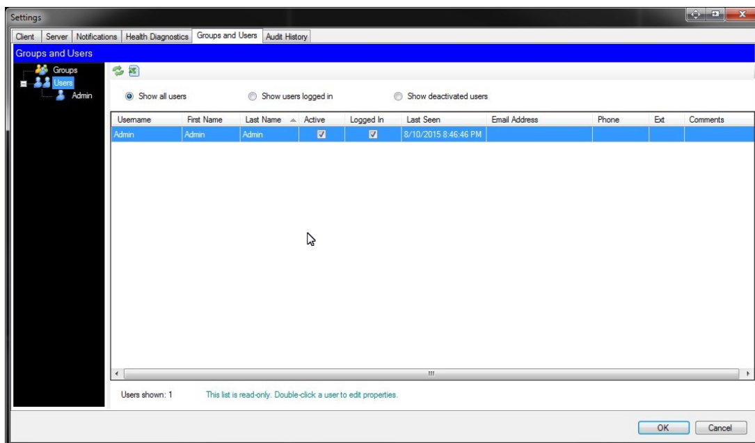
Figure 52: Users Window
