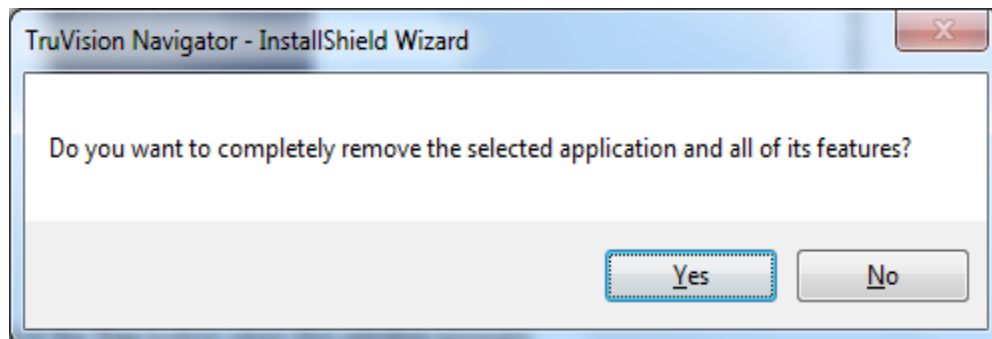
Figure 13: Confirmation window
