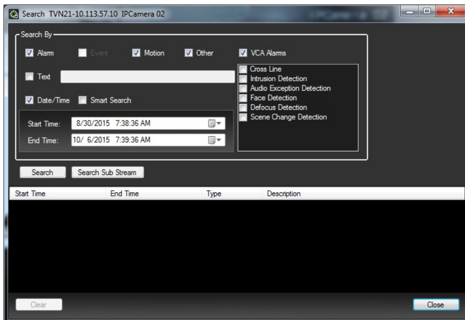
Figure 39: Search dialog
