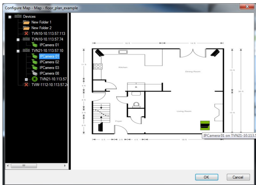
Figure 23: Configure Map
