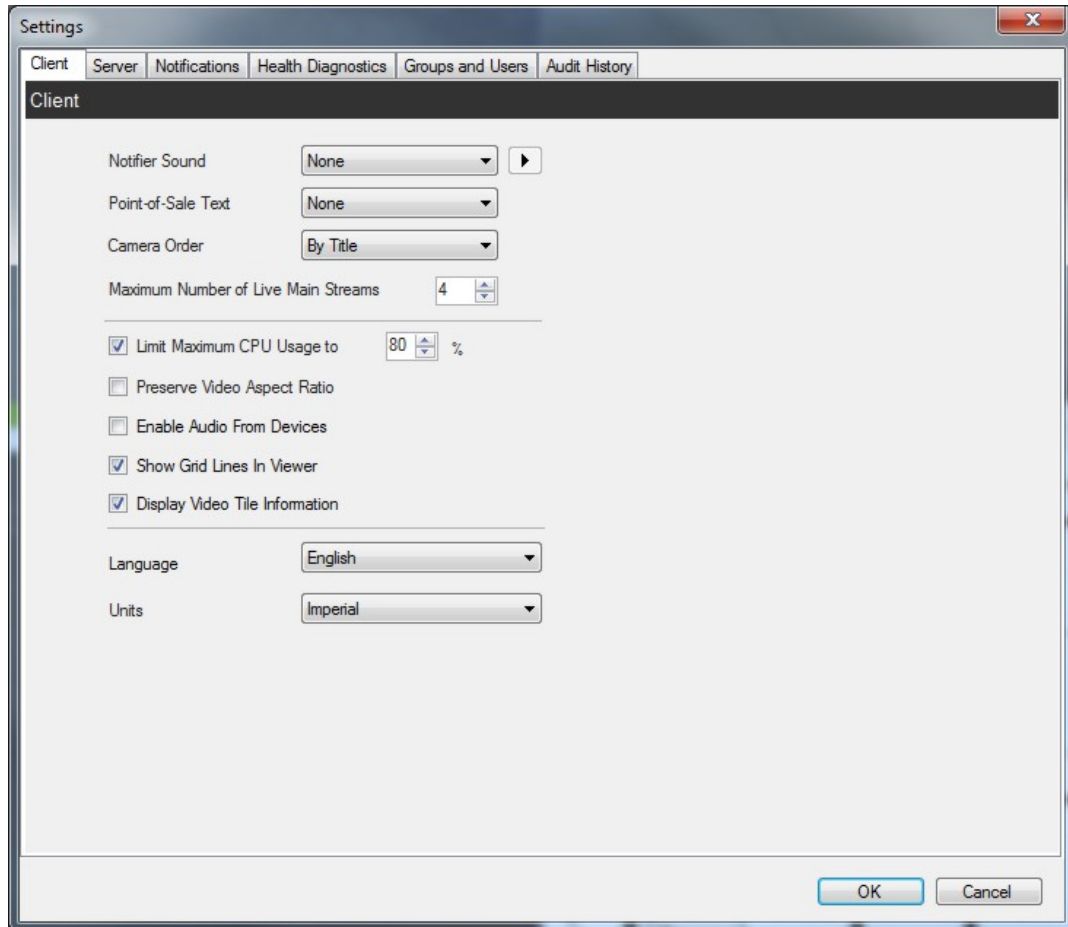
Figure 44: Client Window
