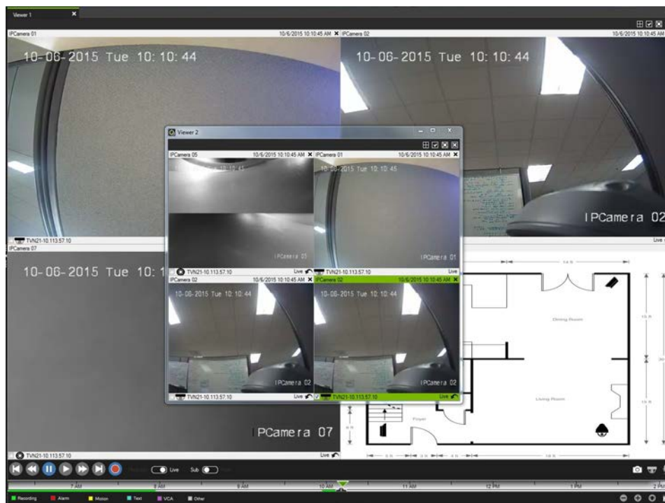
Figure 30: Viewer Panel
