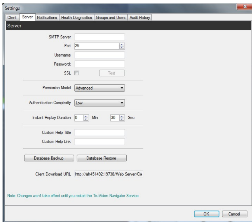
Figure 45: Server window
