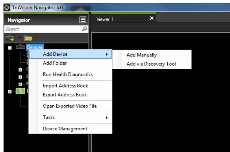
Figure 21: Navigator folders
