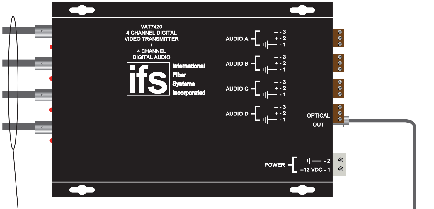
4 BNC Cables (Fixed Video Inputs from Cameras)
