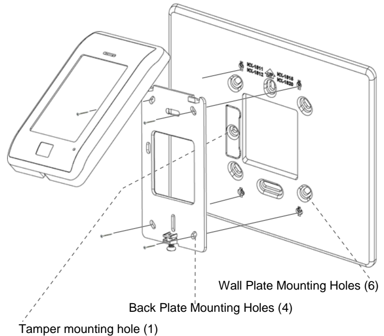
Figure1. Wall plate, with example NX-1820E back plate and NX-1820E Touch Screen
