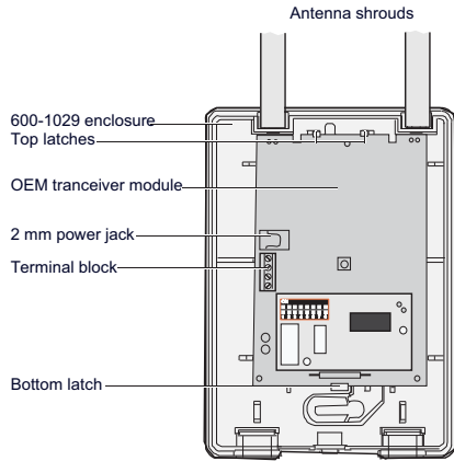
Figure 4: OEM transceiver module mounted in the 600-1029 enclosure
