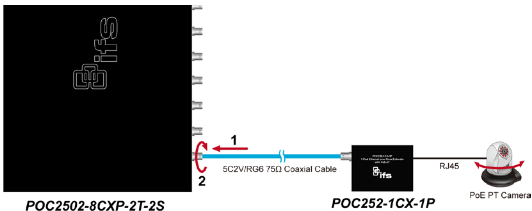
Figure 2-1-8 How to insert the coaxial cable from POC Managed Switch
