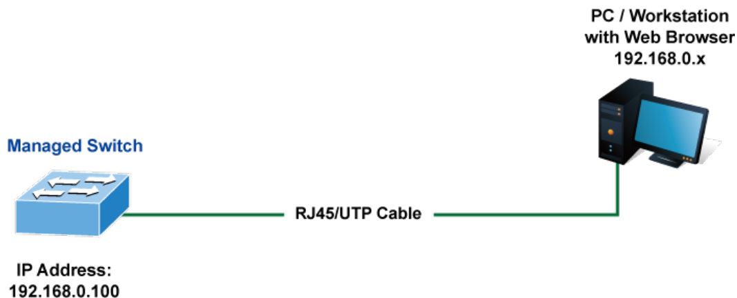
Figure 4-1-1 Web Management
