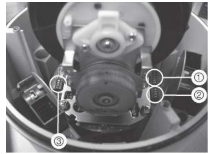
1. Address switches; 2. Baud switches; 3. Protocol switches
