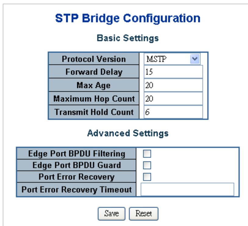
Figure 4-7-7 STP Bridge Configuration page screenshot
