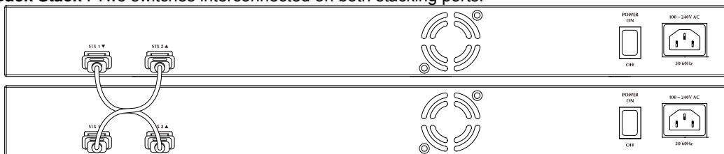
Figure 4-17-3 Back to back Stack topology
