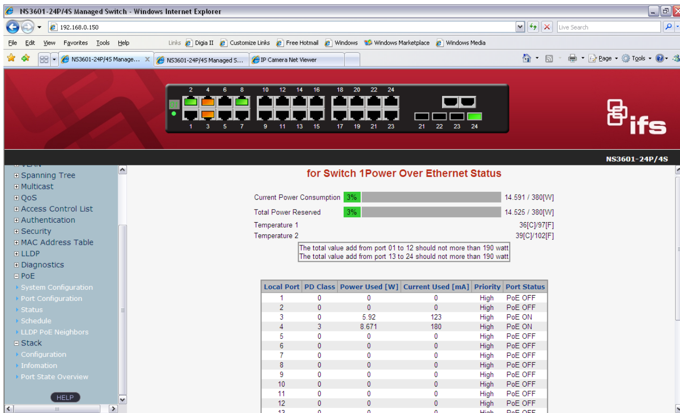
Figure 4-16-4 PoE Status screenshot
