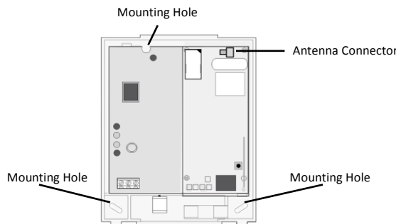
Figure 3: Antenna connector and mounting holes
