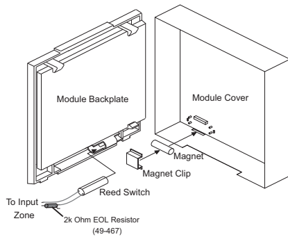
Figure 8: Installing the reed switch
