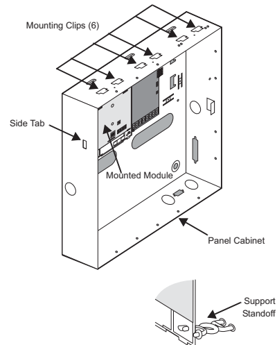
Figure 4: Mounting the module in a Concord, Concord 4, or Concord Express (v4) cabinet
