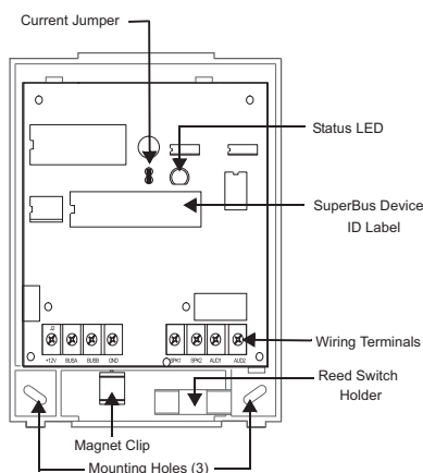
Figure 1: Voice module components and mounting holes
