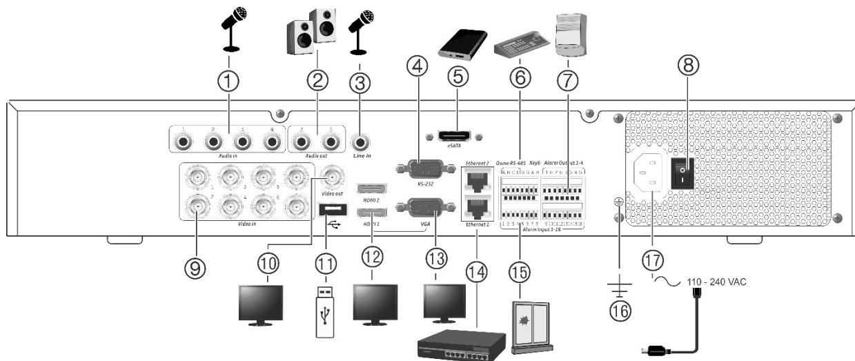
Figure 2: TVR 45HD back panel connections (8-channel models shown)
