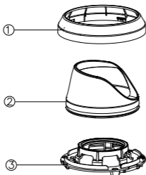
Figure 8: IP turret camera
