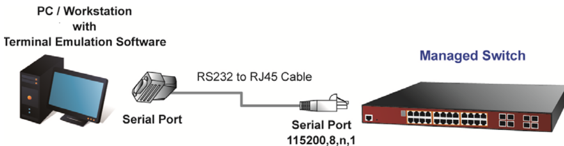
Figure 2-1 Managed Switch Console Connectivity
