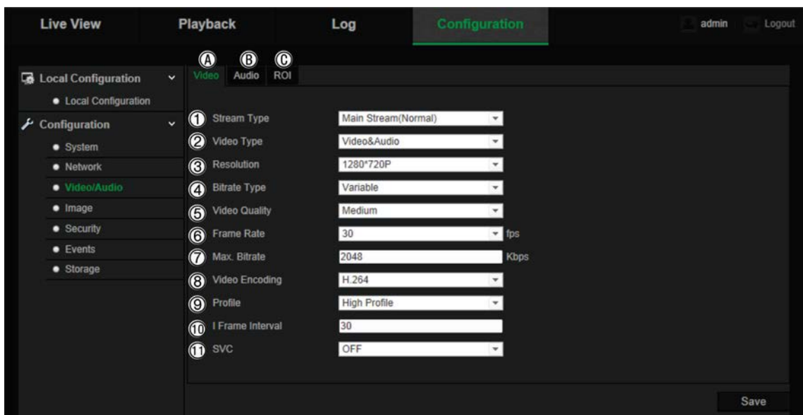
Figure 5: Video/Audio Settings menu (Video tab shown)
