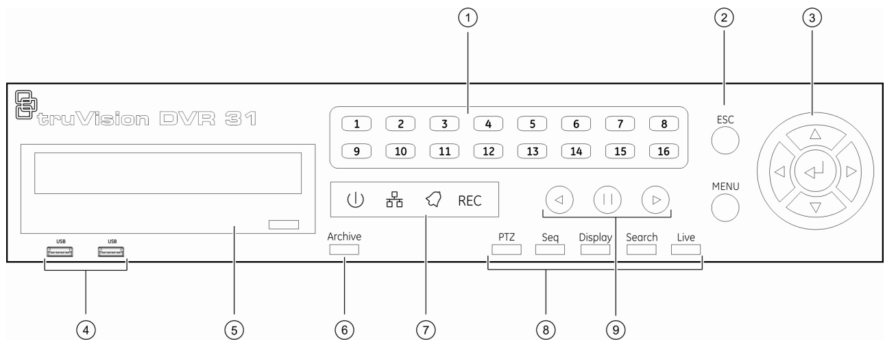
Figure 2: Front panel
