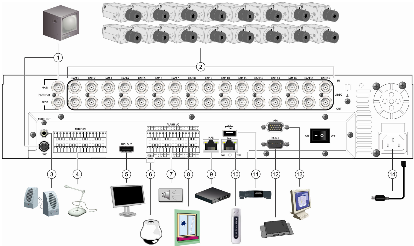
Figure 1: DVR 31 back panel connection diagram
