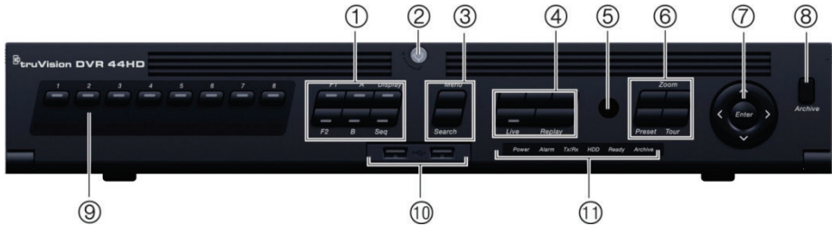
Figure 2: Front panel controls (8-channel model shown)
