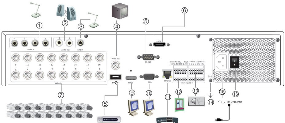
Figure 1: Back panel connections (16-channel model shown)
