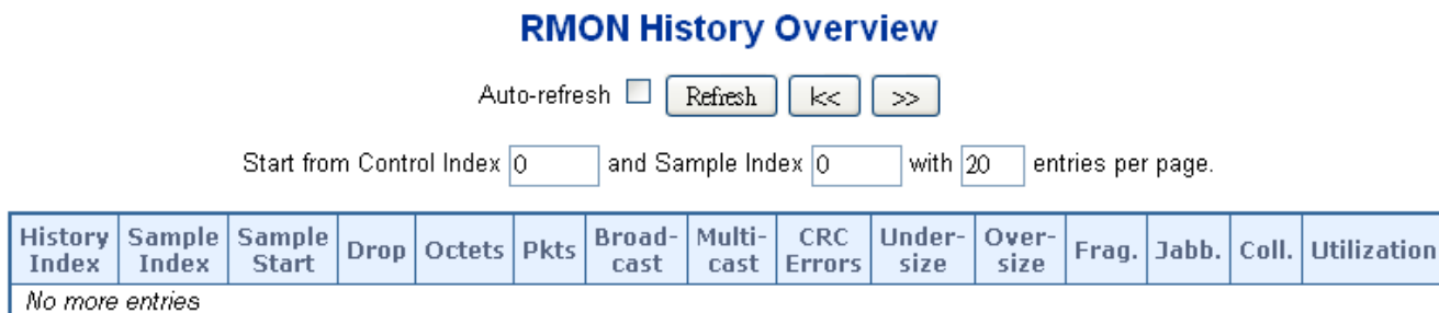
Figure 4-17-6: RMON history overview page screenshot
