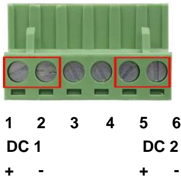
Figure 2-4 6-Pin Terminal Block Power Wiring Input
