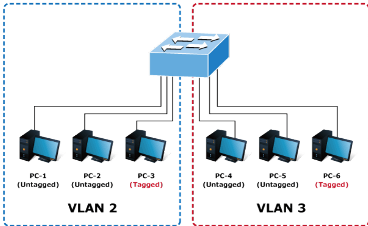
Figure 4-6-8: Two Separate VLAN Diagrams
