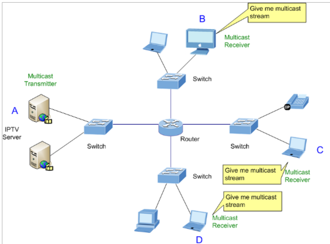
Figure 4-8-1: Multicast Service
