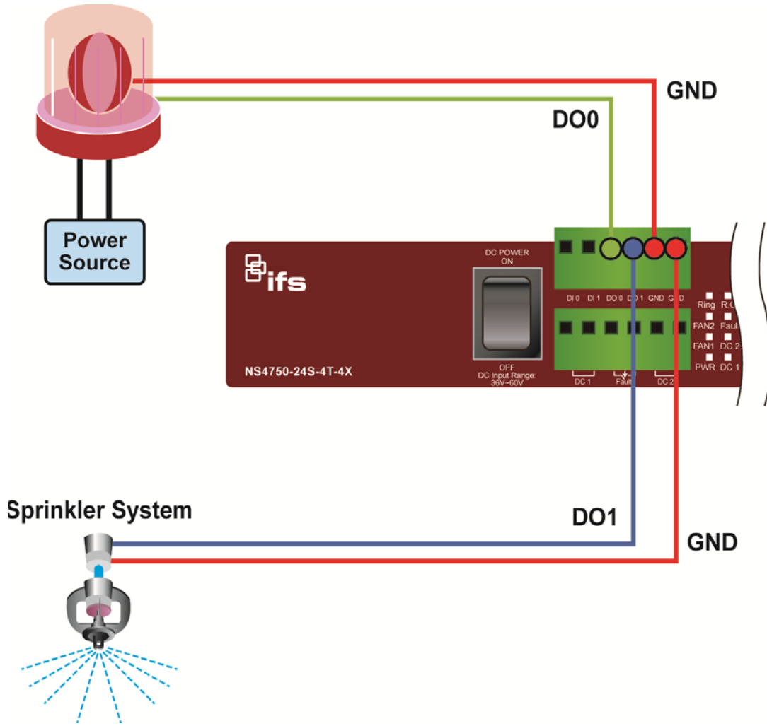
Figure 2-8 Wires DO0 and DO1 to Open Detector
