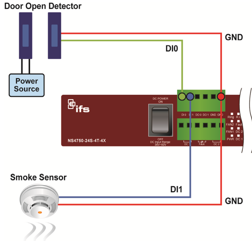
Figure 2-7 Wires DI0 and DI1 to Open Detector
