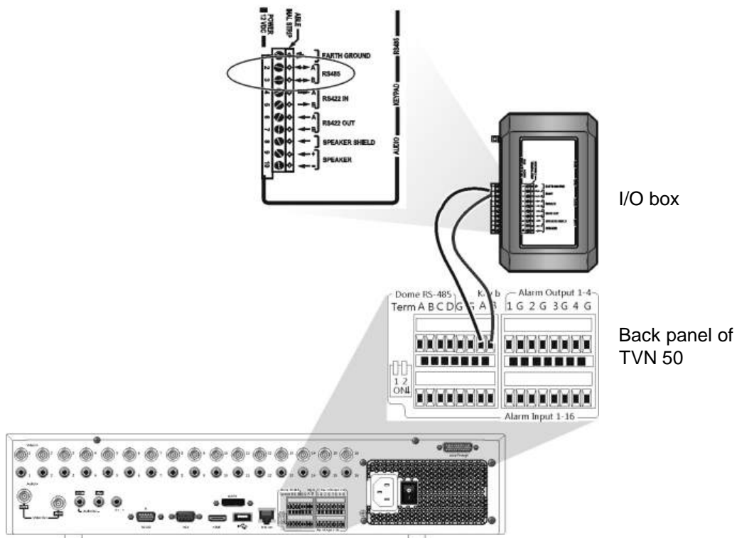
Figure 40: Keypad and NVR connections
