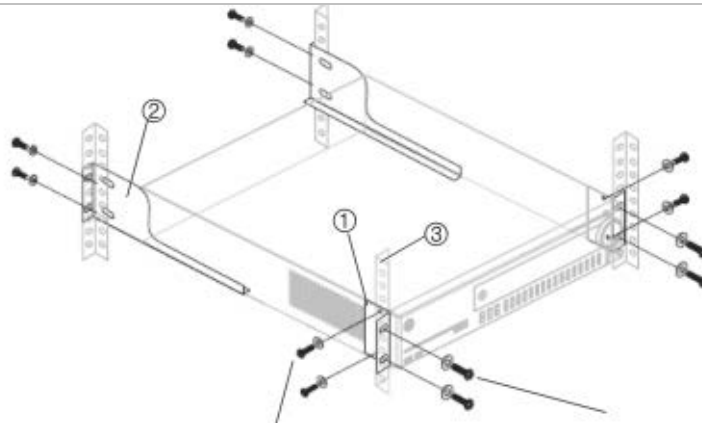
Figure 6: Rack-mount installation
