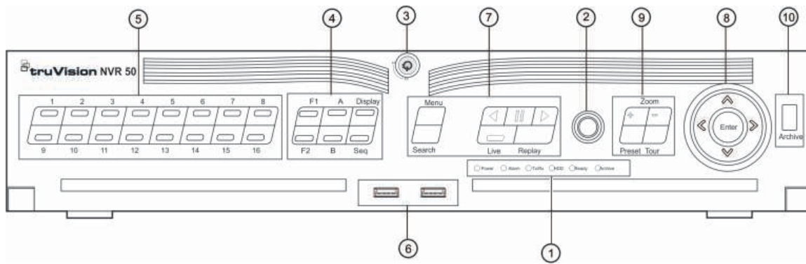
Figure 7: Front panel
