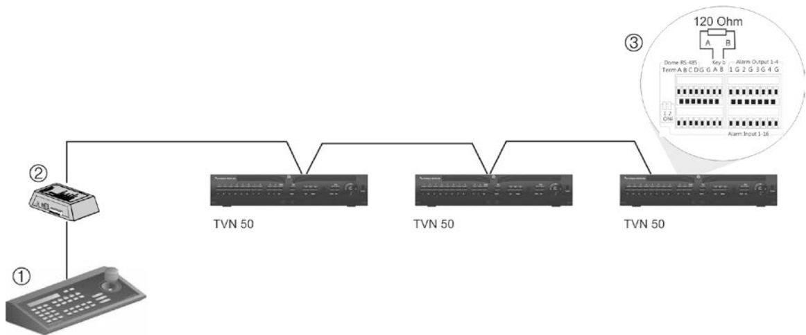
Figure 2: RS-485 bus serial wiring (KTD-405 keypad shown)
