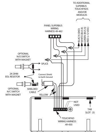
Figure 4: Wiring the touchpad to Advent panels
