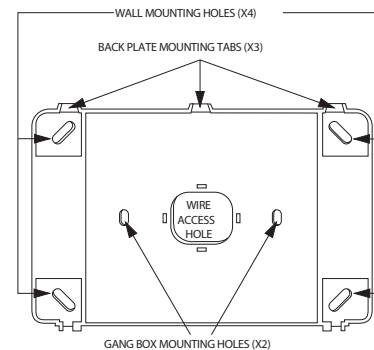
Figure 2: Back plate and mounting holes
