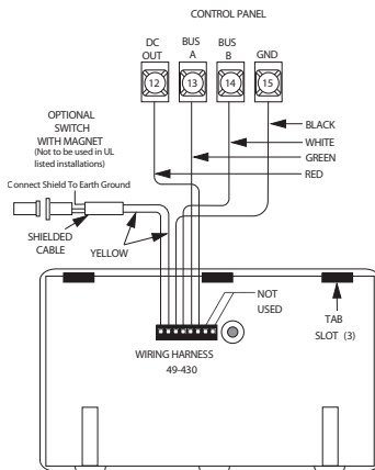
Figure 5: Wiring the touchpad to Ultragard panels
