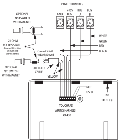
Figure 3: Wiring the touchpad to Concord and Concord Express panels
