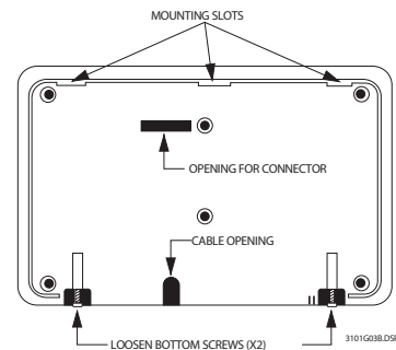
Figure 1: Touchpad mounting slots
